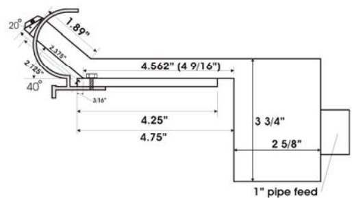
Mounted in Vinyl Liner aluminum coping
