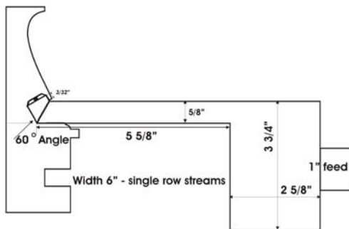
Cantilever form for concrete coping/deck
