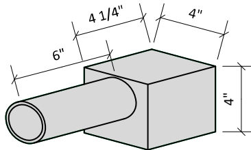
Round Nozzle
