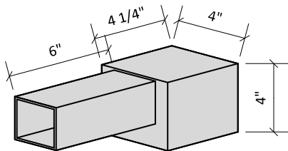
Square Nozzle
