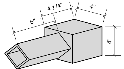
Diagonal Nozzle
